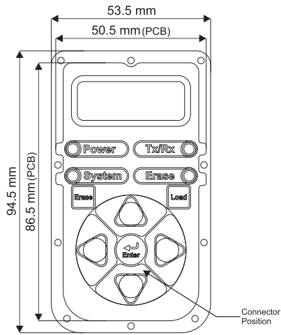
Mechanical Drawing
