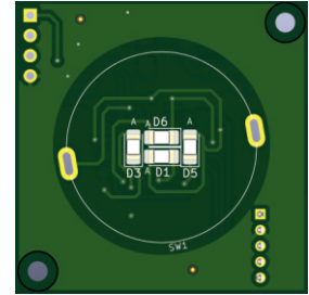
Size 32.0 x 32.0mm with spring
