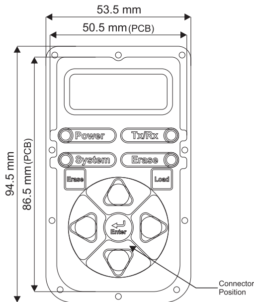
Mechanical Drawing
