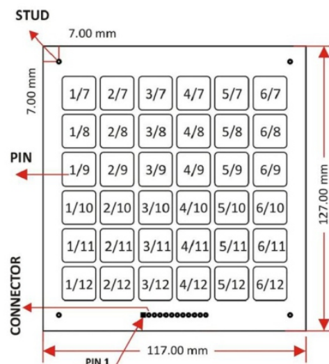
FRONT VIEW (Keys Matrix)
