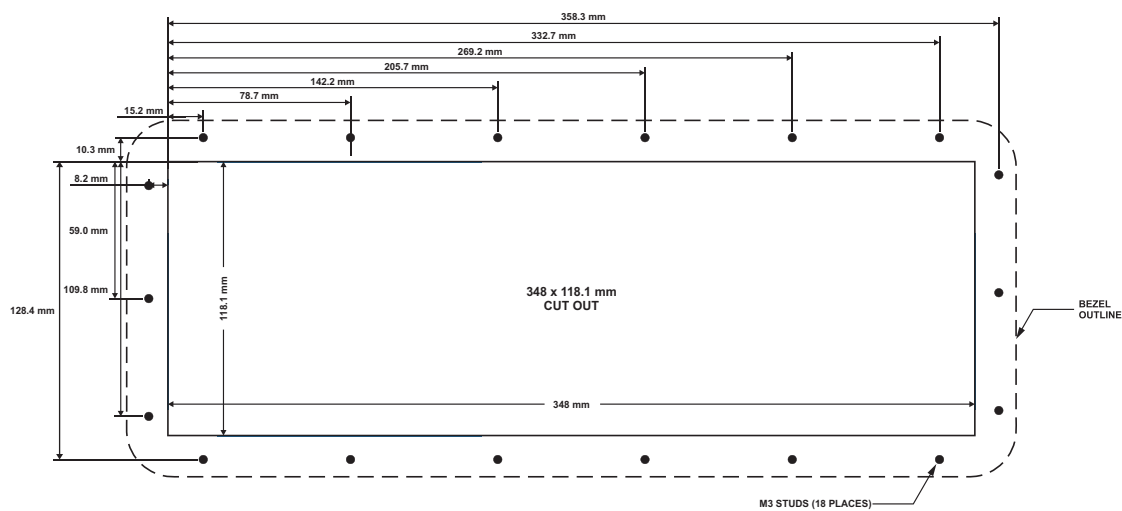
BOTTOM VIEW
