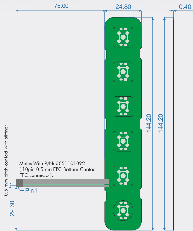
Printed Circuit Board
