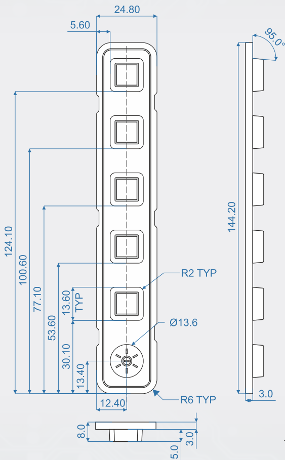
Rubber Mechanical Drawing
